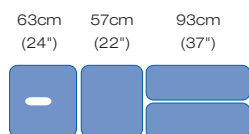
Model 2142A - split leg Model 2162A - split leg with drainage
